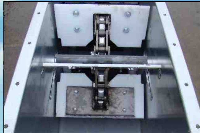
Each UHMW paddle bolts onto a large, formed steel backer plate that is welded onto the chain.
