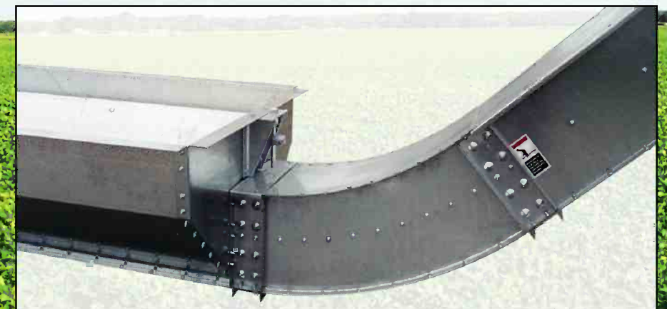
Long radius, high flow bend sections with optional bottom AR steel liners.
